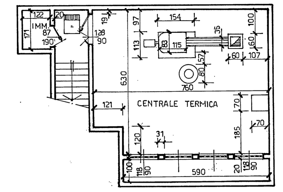
PIANO CANTINATO
